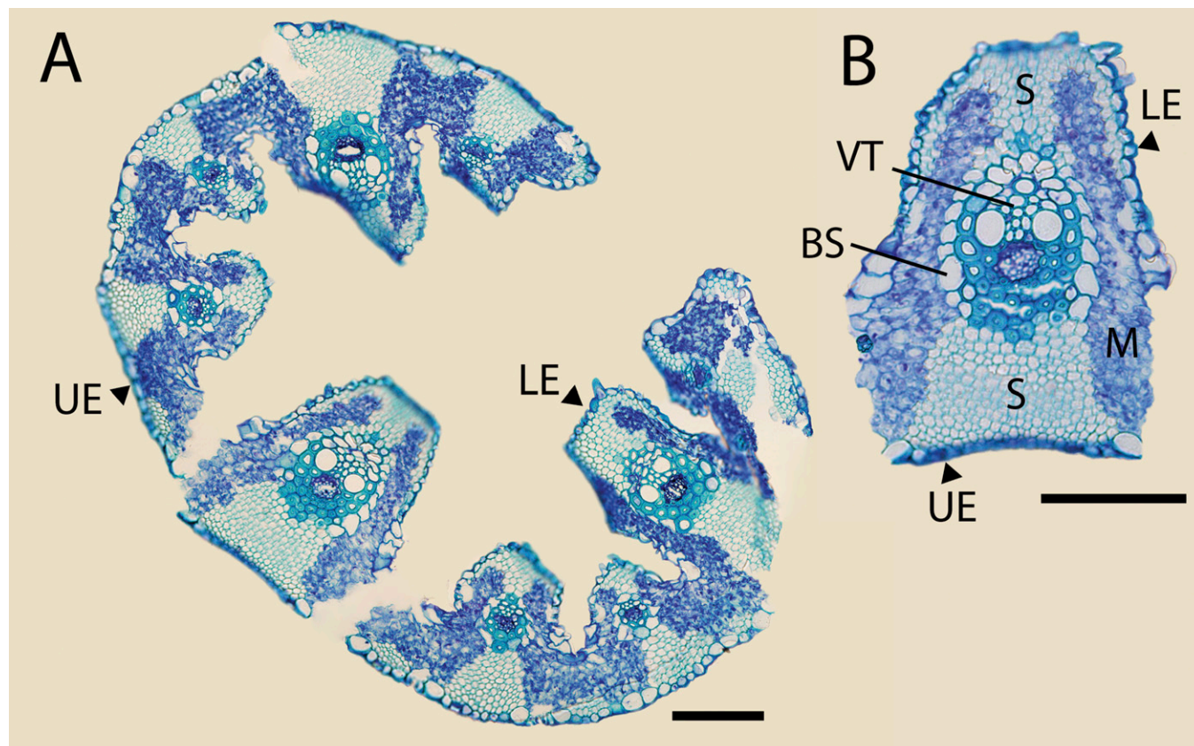
FIG. 4. Leaf cross sections of Sartidia isaloensis demonstrating anatomy typical of a C 3 species: many mesophyll cells between a few large veins. A. Cross section of leaf blade; scale bar = 100 µm; B. Cross section of a leaf blade margin; scale bar = 100 µm. BS = Bundle Sheath; M = Mesophyll; LE = Lower Epidermis; UE = Upper Epidermis; S = Sclerenchyma; VT = Vascular Tissue. Material from the type collection Razanatsoa et al. 578 (K).
