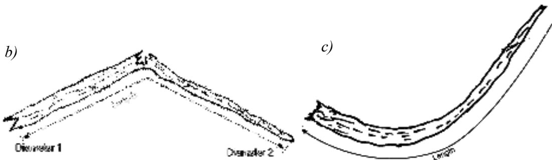
Figure 26. Dead-wood measurements
