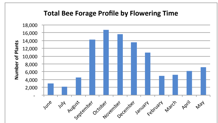
Figure 25. Case Study: bee forage profile for combined plantings of both pre-existing and proposed.
