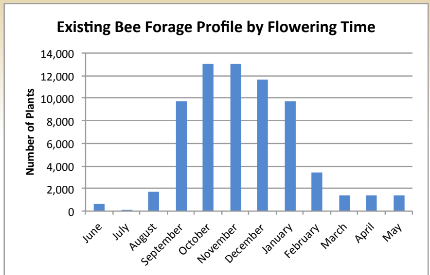
Figure 23. Case Study: bee forage profile for existing riparian planting.
