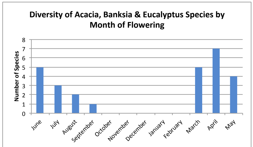
Figure 14. Species diversity chart of Acacia, Banksia and Eucalyptus species by month of flowering.
