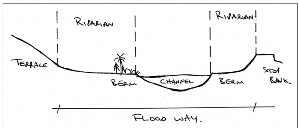
Figure 16. Riparian zones.
