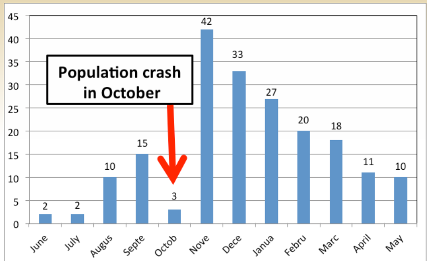
Figure 21. Hypothetical example of a Bee Forage Profile: This bee forage profile chart shows the number of plants from different species that are flowering in each month of the year for one foraging area. This bee forage profile illustrates a serious deficit in October just after two months of spring build-up have occurred.
