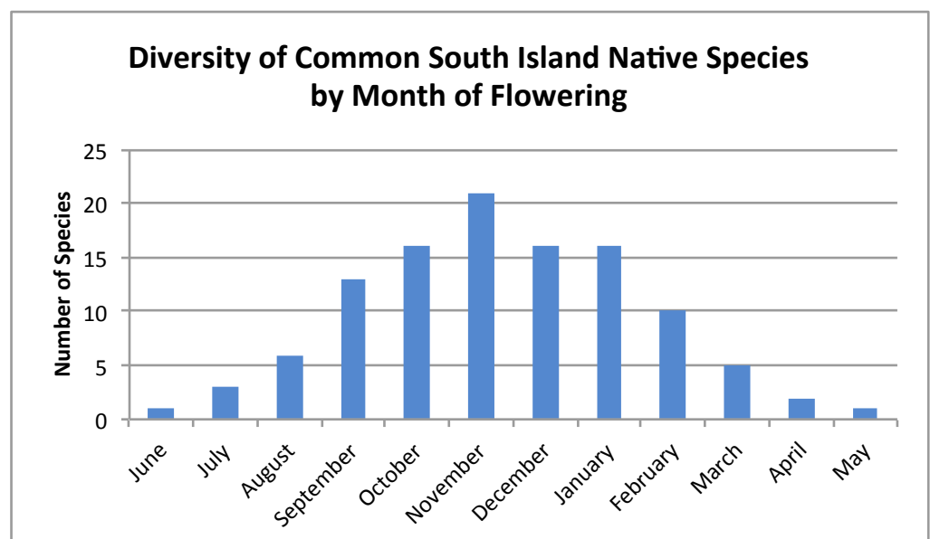
Figure 10. Species diversity chart for the most widely used South Island native bee species by month of flowering.
