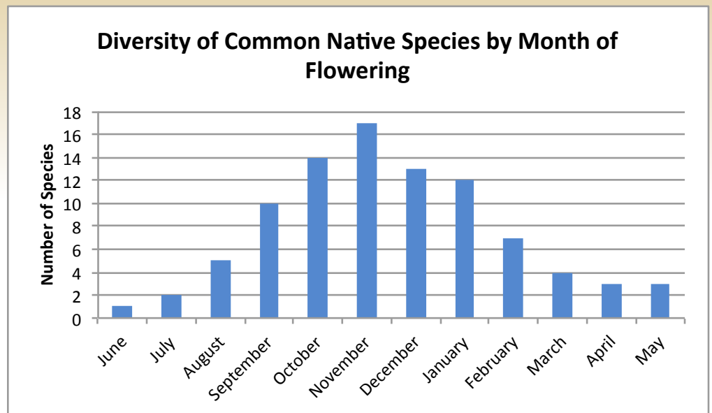
Figure 8. Species diversity chart for most widely used native riparian bee species by month of flowering.
