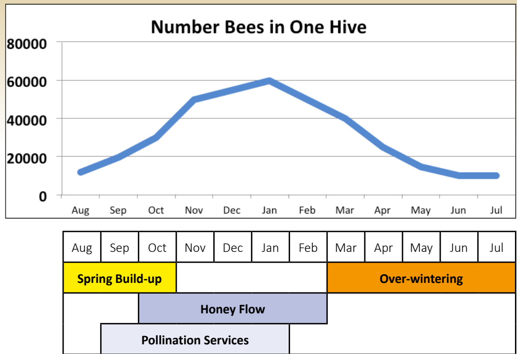
Figure 32. Bee colony population size and annual cycle showing pollen and nectar demand and typical activities for each season.
