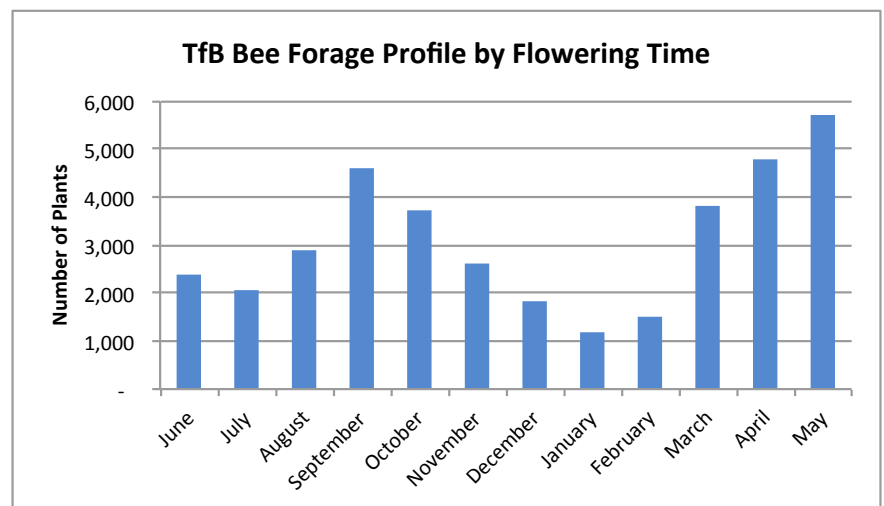
Figure 24. Case Study: bee forage profile for proposed planting.
