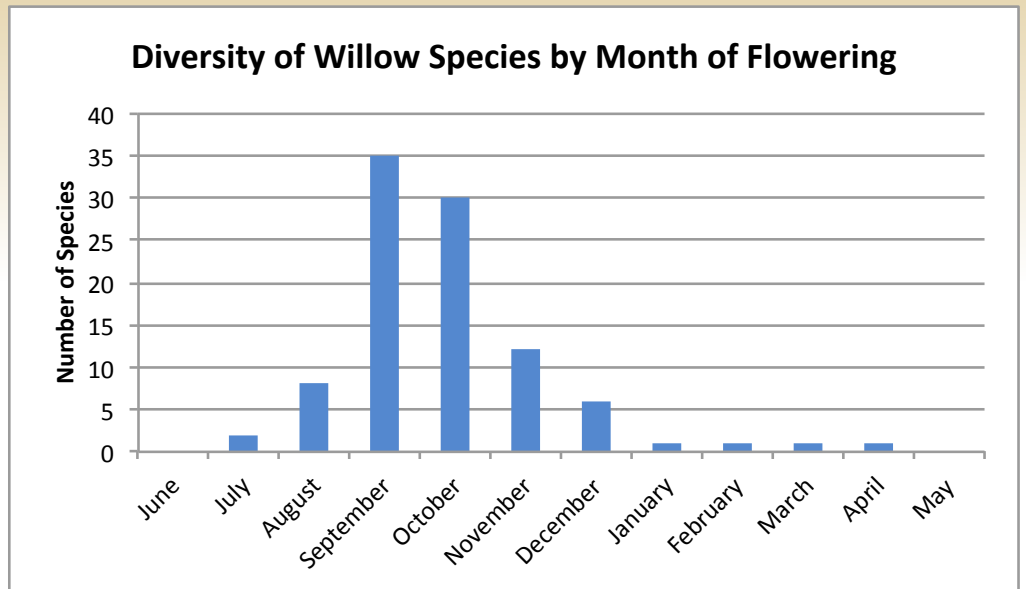
Figure 11. Diversity chart for willow species by month of flowering.
