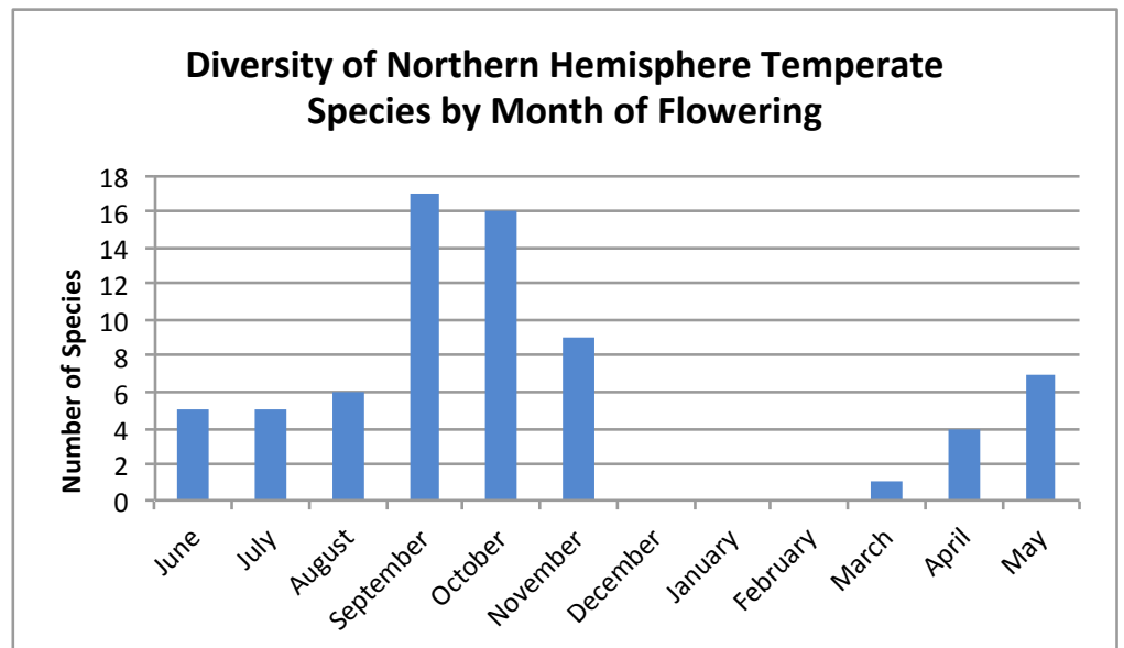
Figure 15. Species diversity chart of Northern Hemisphere temperate species by month of flowering.
