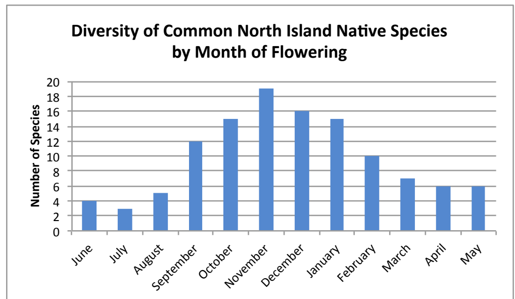
Figure 9. Species diversity chart for the most widely used North Island native bee species by month of flowering.
