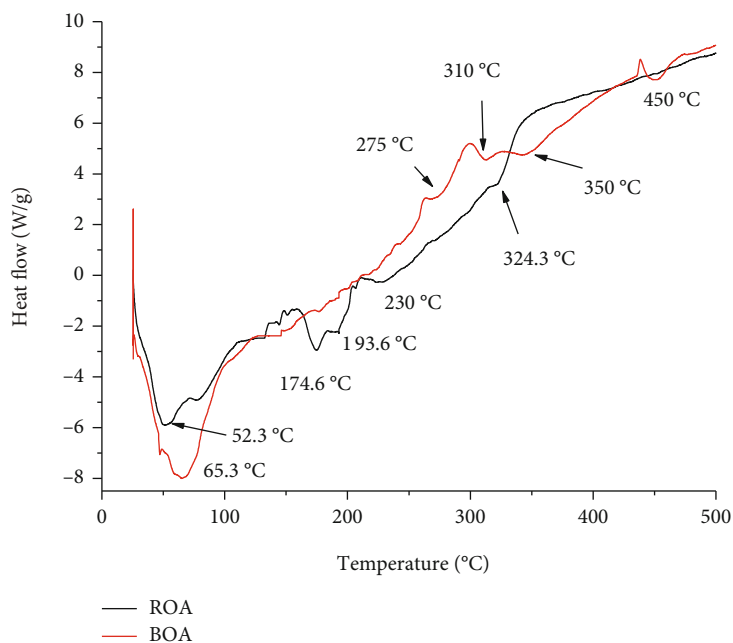
FIGURE 11: DSC image of ROA and BOA fibers.
