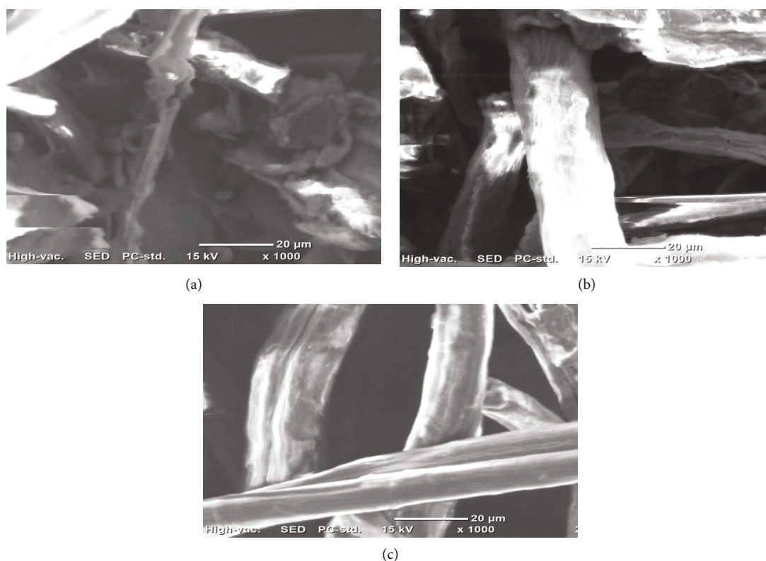
FIGURE 6: SEM image of ROA (a), AOA (b), and BOA (c).
