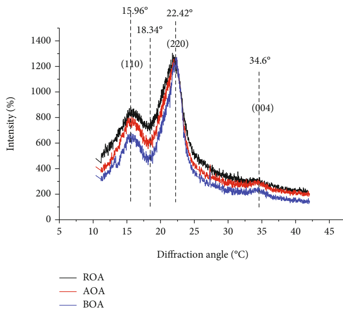
FIGURE 8: XRD pattern of ROA, AOA, and BOA.
