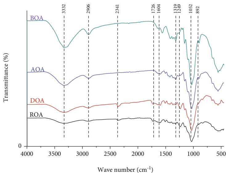
FIGURE 7: FTIR spectra of ROA, DOA, AOA, and BOA.
