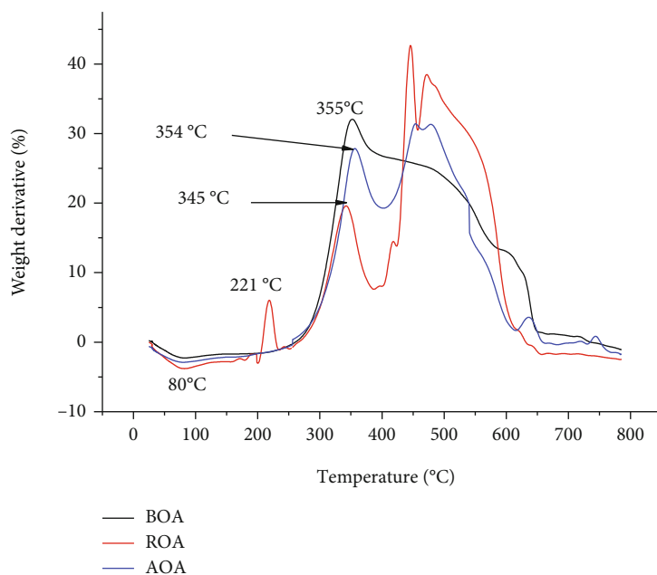
FIGURE 10: DTA curve of ROA, AOA, and BOA fibers.
