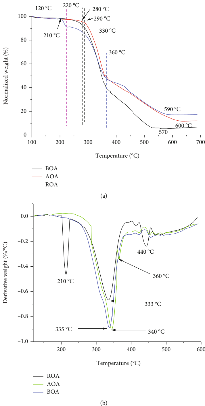
FIGURE 9: Normalized TGA curve of ROA, AOA, and BOA samples (a) and their DTG peaks (b).
