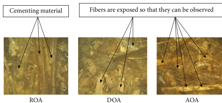
FIGURE 4: Optical microscope image of untreated (ROA), dewaxed (DOA), and alkali-treated (AOA) Oxytenanthera abyssinica fiber.
