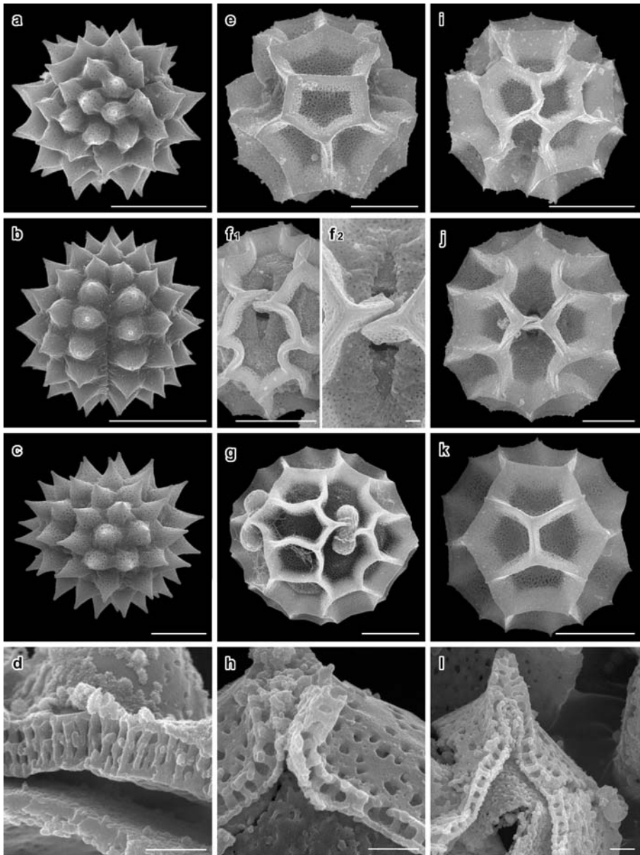
Fig. 6 SEM views of Arctotideae pollen. a, b, d Haplocarapha scaposus . c Haplocarapha nervosa . a Polar; b apertural; c equatorial; d fractured grain, showing well developed horizontal internal tectum and cavea. e Gazania rigens . f1, g, h G. krebsiana . f2 Gazania longiflora . e Polar view, showing large lacunae with highly perforated surface. f1 Apertural view, showing unequal arms of lophae directly over pore opening with left portion of ridge always over the right portion (compare with unacetolysed equivalent, g ); f2 , higher magnification of lophae at aperture (scale bar 1 \mu\text{m} ); g equatorial view of unacetolysed grain, showing non-resistant aperture plugs between the lophae at aperture; h fractured grain showing single columellae layer and portion of cavea. Note striking difference in columellae structure from previously fractured grains. i, k Gorteria diffusa . j, l Gorteria personata . i Polar view; j aperture, showing left lophae over right in pore region; k lateral view showing aperture with left-over-right arrangement of lophae; l fractured grain. Scale bars: whole grains, 10 \mu\text{m} (except f2 , see above); fractured grains, 1 \mu\text{m}
