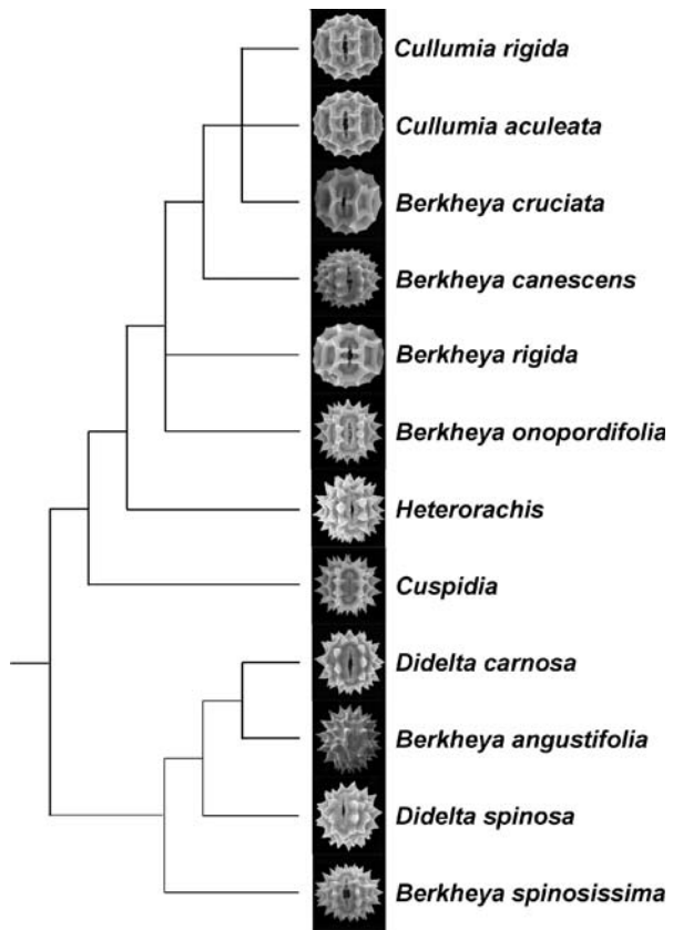
Fig. 14 Phylogeny of DID and BER clades of Gorteriinae based on molecular data (modified from Funk et al., 2004) showing distribution of sub-lophate and lophate pollen grains
