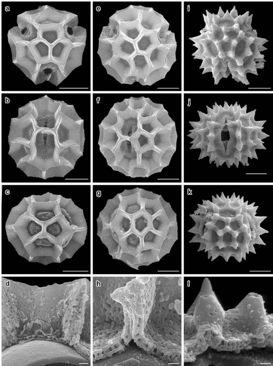
Fig. 7 SEM views of Arctotideae pollen. a, c, d Hirpicium bechuarensense . b H. echinus . a Polar; b aperture, showing left lophae over right in pore region; c lateral, showing lophae on left and right margins of pollen grain; d fractured grain. e–h H. integrifolium . e Polar, note greater number of lacunae than in previous taxa; f aperture, showing left lophae over right in pore region; g equatorial; h fractured grain. i–l B. spinosissima . i Polar; j apertural; k equatorial; l fractured grain, showing single columellae layer with weakly developed horizontal internal tectum above a cavea. Scale bars : whole grains, 10 \mu\text{m} ; fractured grains, 1 \mu\text{m}
